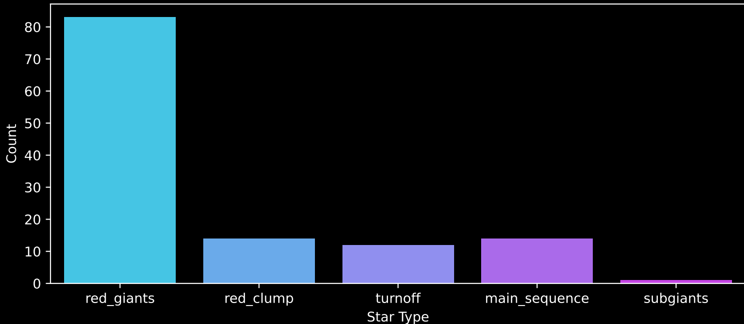
APOGEE DR17 Field: [SMC11] Count plot of Star Type
