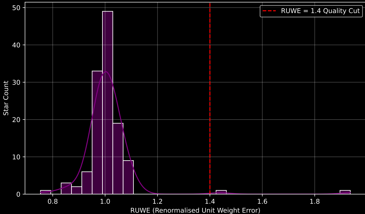
GAPOGEE DR17 Field [SMC11] RUWE Distribution (n= 124)
