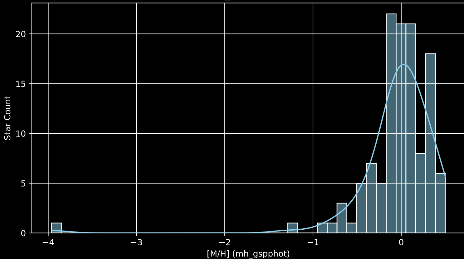
APOGEE DR17 Field: [SMC11 [M/H] (mh_gspphot) (n= 121)
