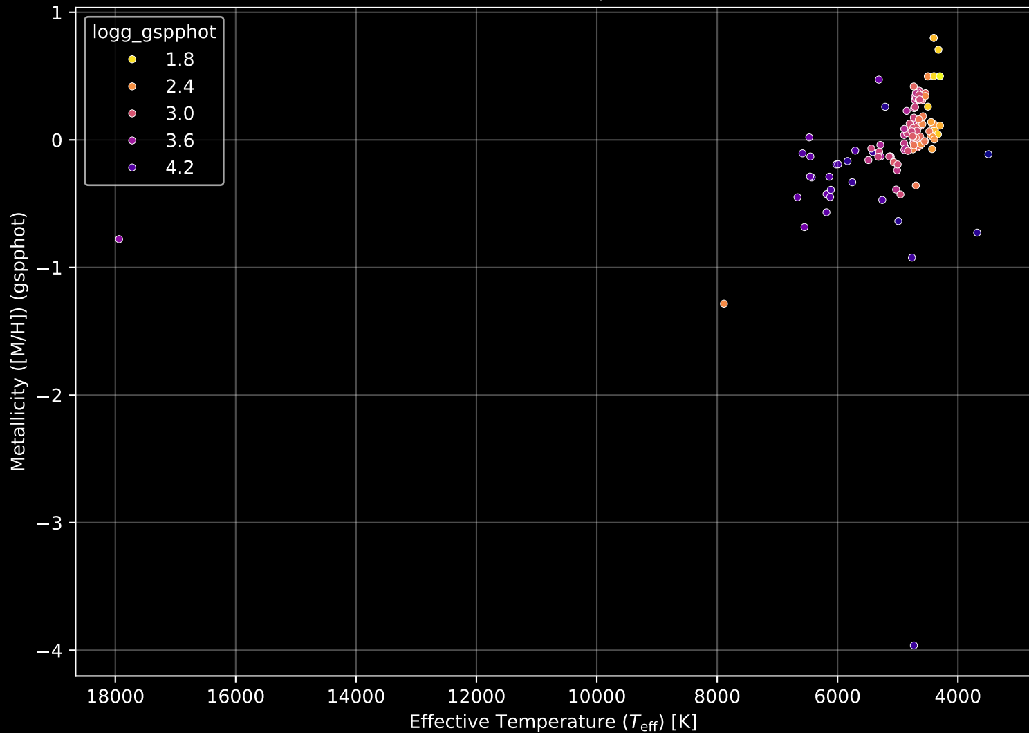
APOGEE DR17 Field: [SMC11] Stellar Population Parameters (n= 124)
