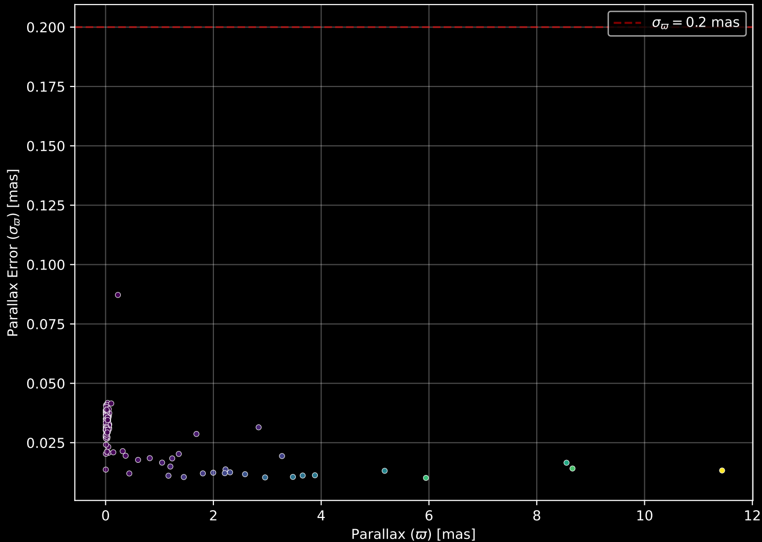
APOGEE DR17 Field: [SMC11] Parallax Quality (n= 124)
