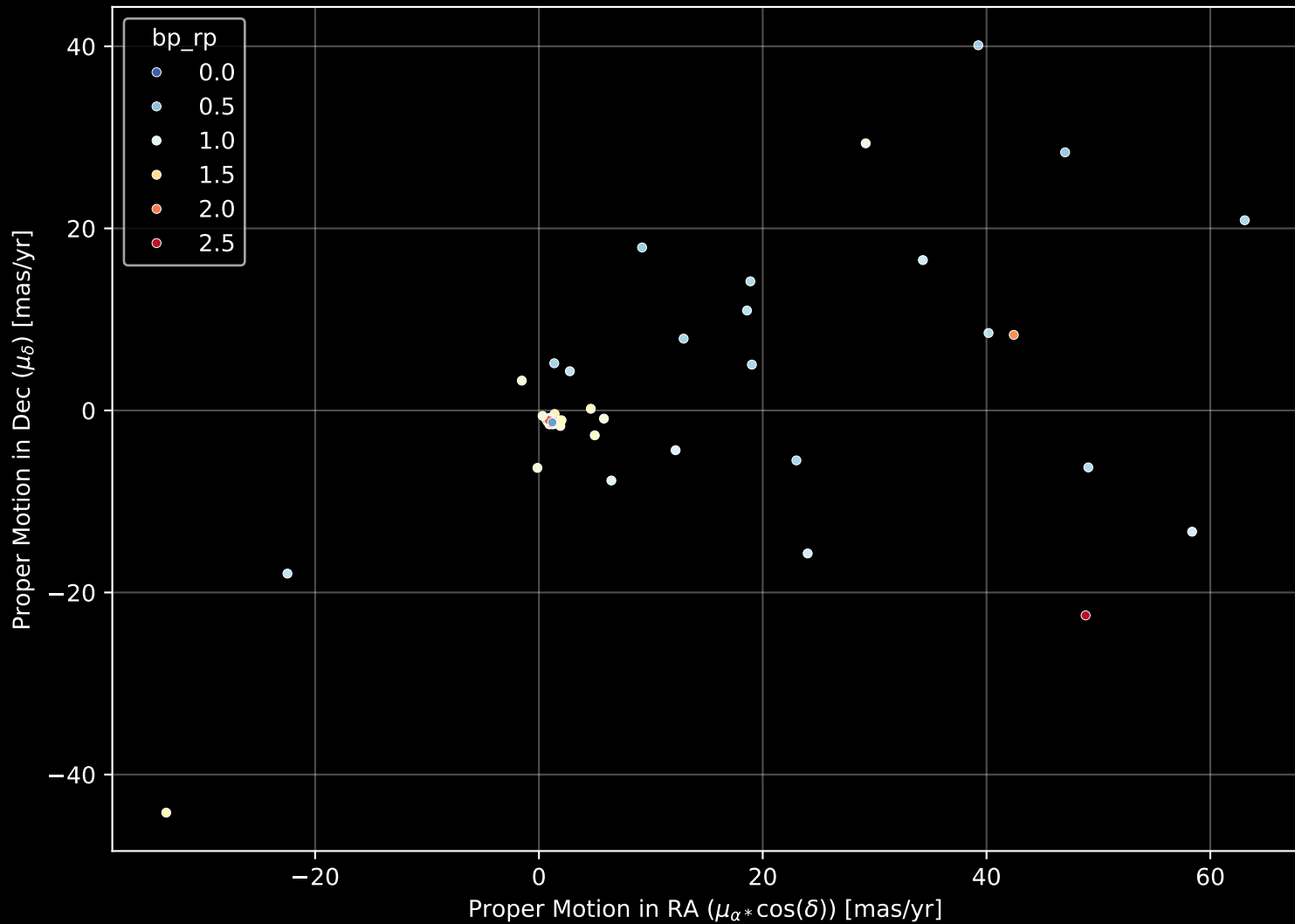
APOGEE DR17 Field: [SMC11] Proper Motion Diagram (n= 124)
